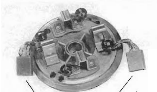
BRUSHES EARTHED TO STARTER END BRACKET
