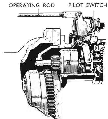
SECTIONED VIEW OF STARTER AND BELL-HOUSING Showing starter operating rod in position
